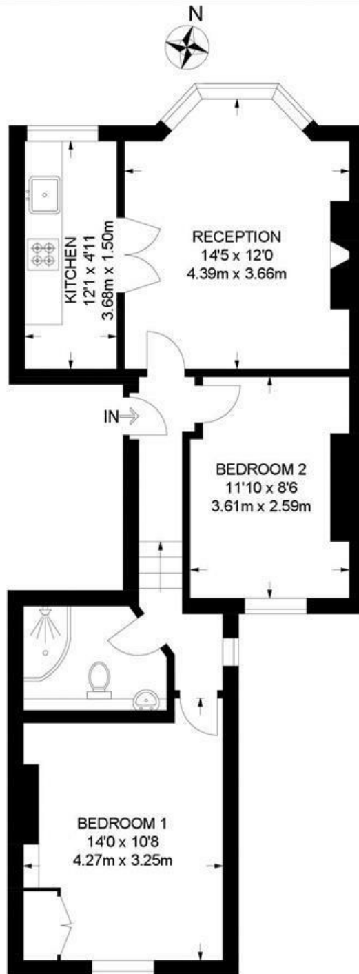
FIRST FLOOR
